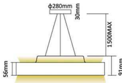
Direct and indirect lighting
